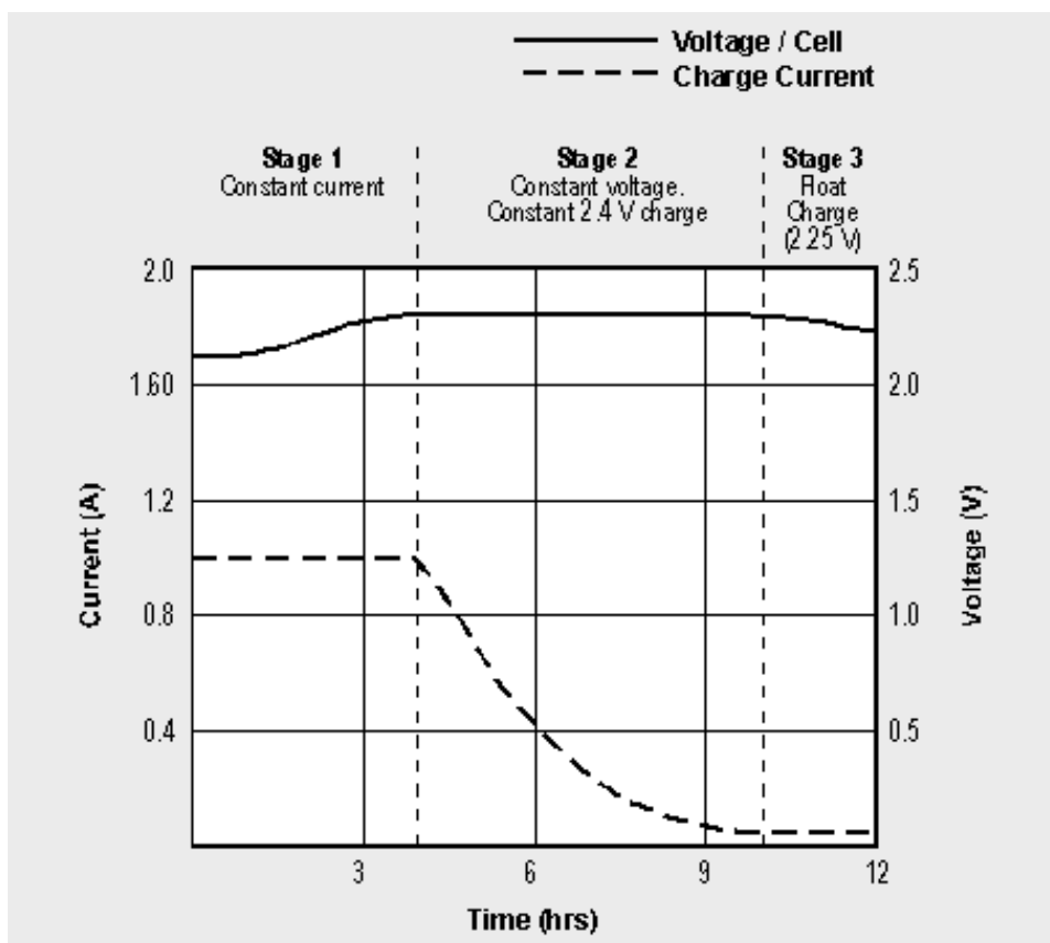
Figure 4-3: Charge stages of a lead acid battery.
