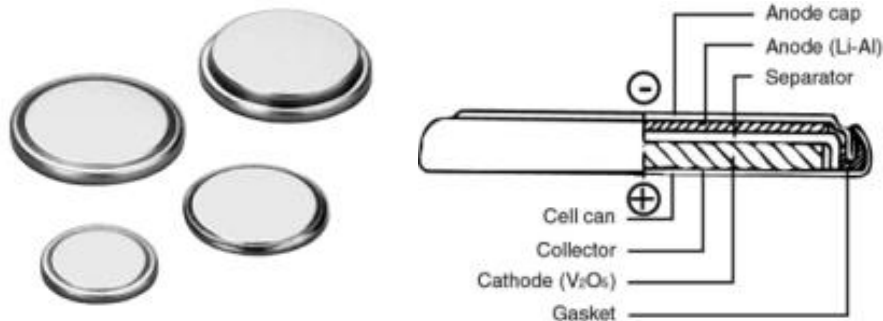
Figure 3-2: The button cell.
