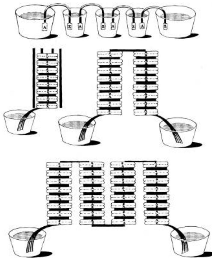
Figure 1-2: Four variations of Volta's electric battery. Silver and zinc disks are separated with moist paper. ©Cadex Electronics Inc.
