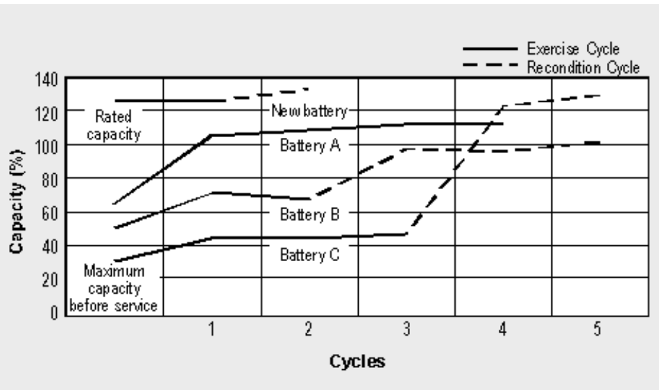
Figure 10-3: Effects of exercise and recondition.
