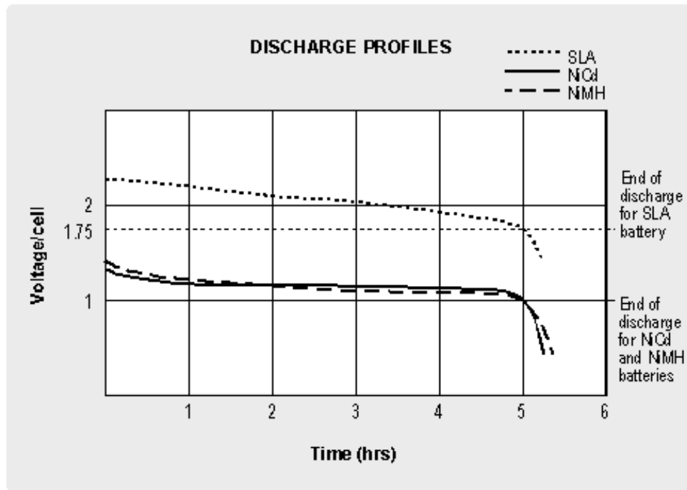
Figure 5-1: Discharge characteristics of NiCd, NiMH and SLA batteries. While voltage readings to measure the SoC are not practical on nickel-based batteries, the SLA enables some level of indication as to the SoC.
