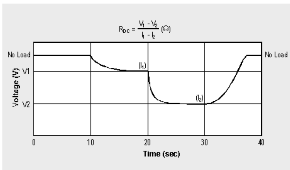
Figure 9-5: DC load test.
