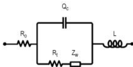
Figure 9-10: Ohmic, inductive and capacitive resistance in batteries.
