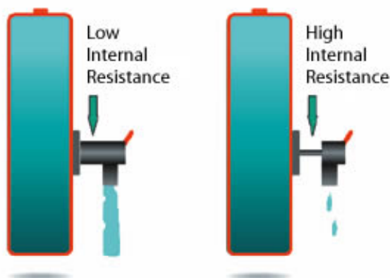
Figure 6-2: Effects of impedance on battery load. A battery with low impedance provides unrestricted current flow and delivers all available energy. A battery with high impedance cannot deliver high-energy bursts due to a restricted path, and equipment may cut off prematurely.
