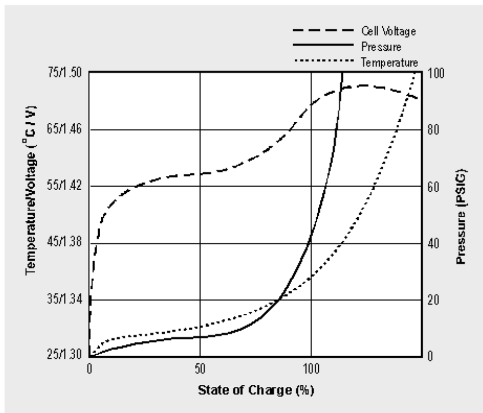
Figure 4-1: Charge characteristics of a NiCd cell. These cell voltage, pressure and temperature characteristics are similar in a NiMH cell.
