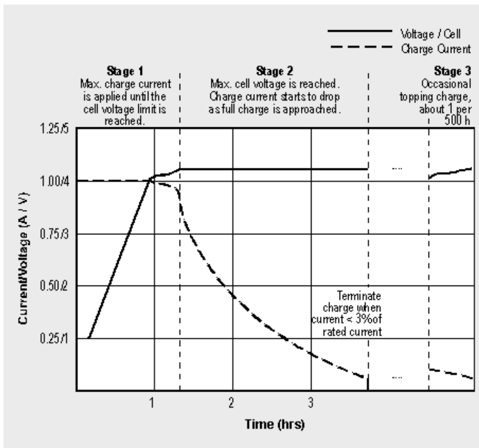
Figure 4-5: Charge stages of a Li-ion battery.
