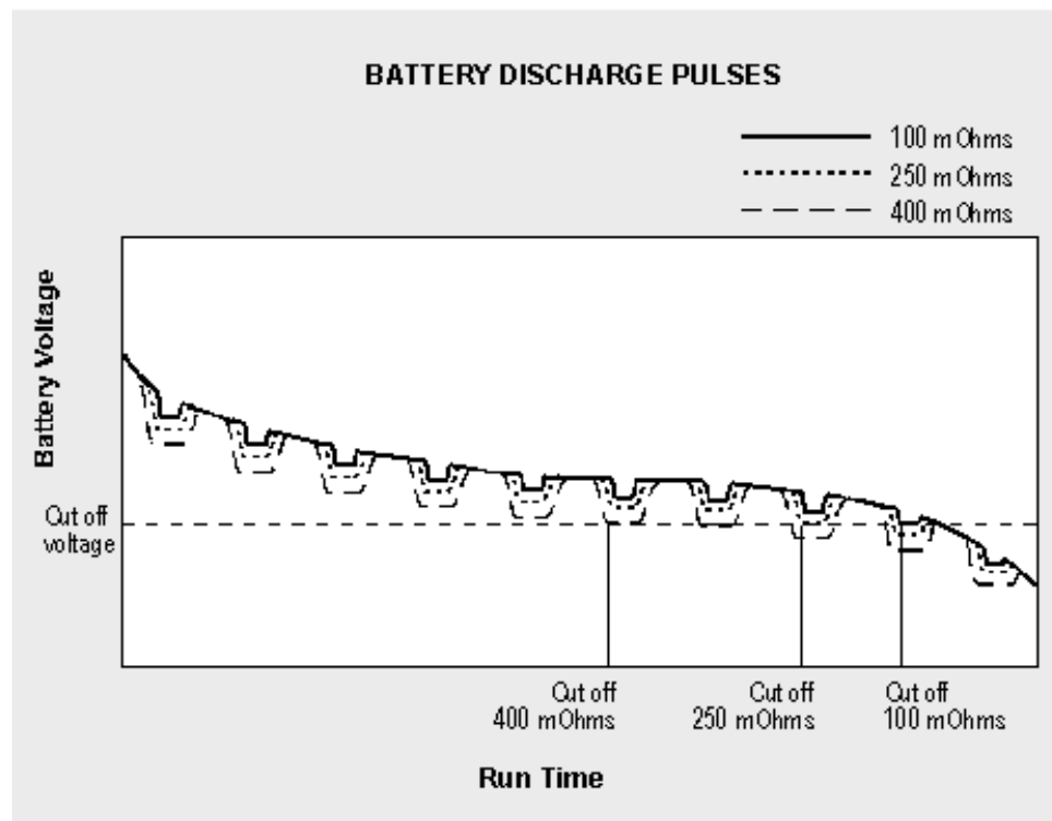
Figure 6-3: Discharge curve.
