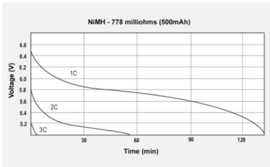
Figure 9-3: Talk-time of a NiMH battery under the GSM load schedule. This battery has 107% capacity and 778m \Omega internal resistance.
