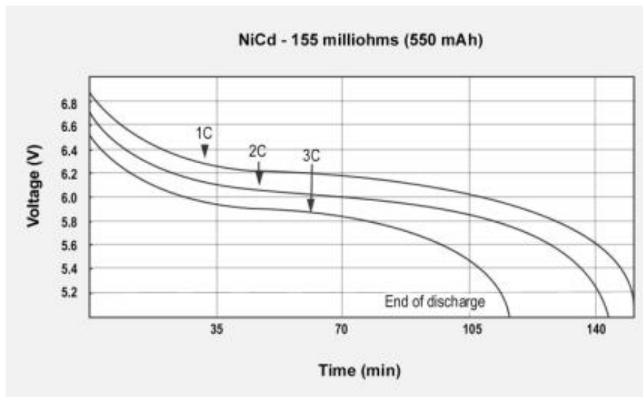
Figure 9-2: Talk-time of a NiCd battery under the GSM load schedule. This battery has 113% capacity and 155m \Omega internal resistance.
