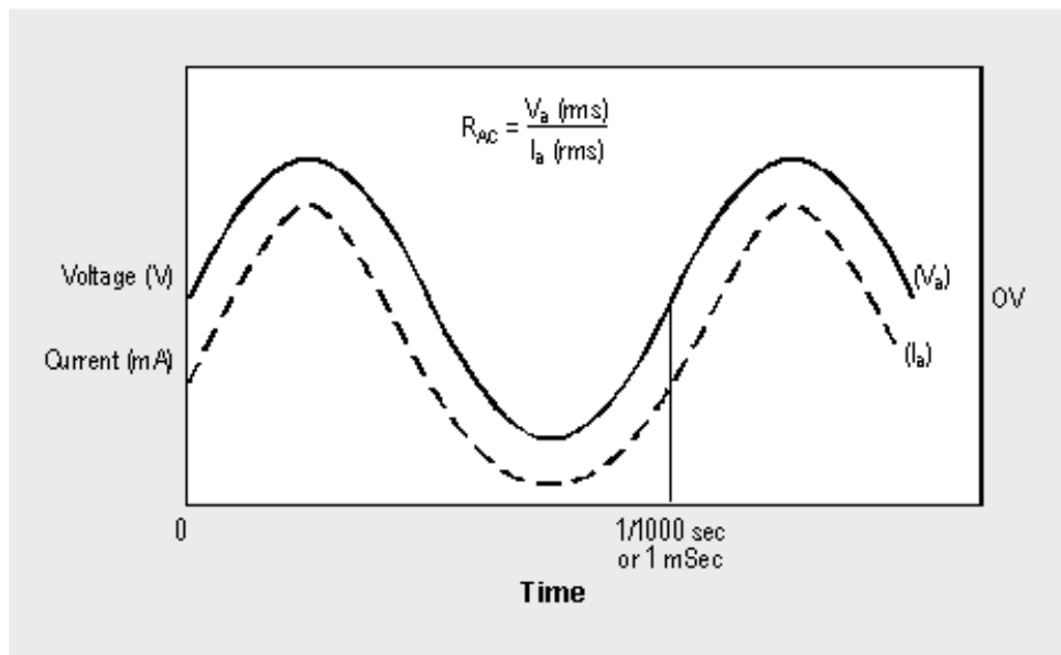
Figure 9-6: AC load test.
