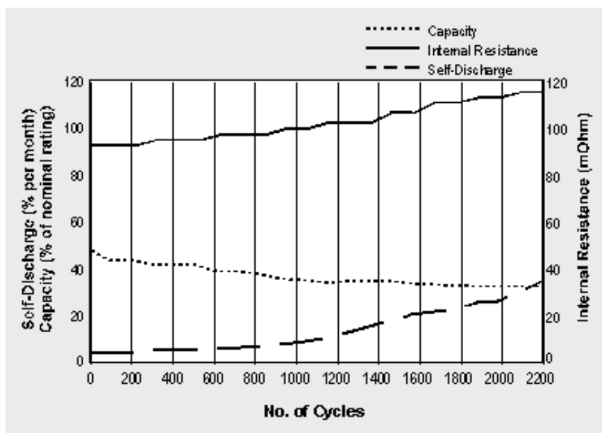
Figure 8-2: Characteristics of a NiCd battery with ultra-high capacity cells. This battery is not as favorable as the standard NiCd but offers higher energy densities and performs better than other chemistries in terms of endurance. This illustrations shows results for a 6V, 700mA NiCd.
