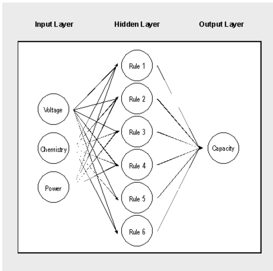
Figure 13-3: Flowchart of a neuro-network based on fuzzy logic. The first three circles on the left are the inputs. The data entering is 'fuzzified'
