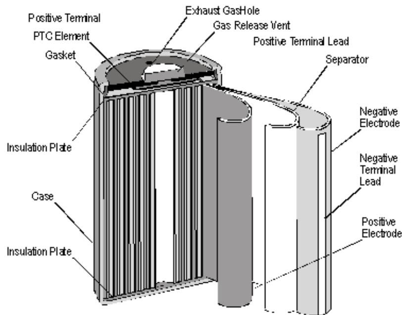
Figure 3-1: Cross-section of a classic NiCd cell.
