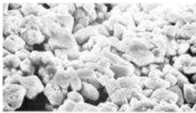
Figure 10-1: Crystalline formation on NiCd cell.
