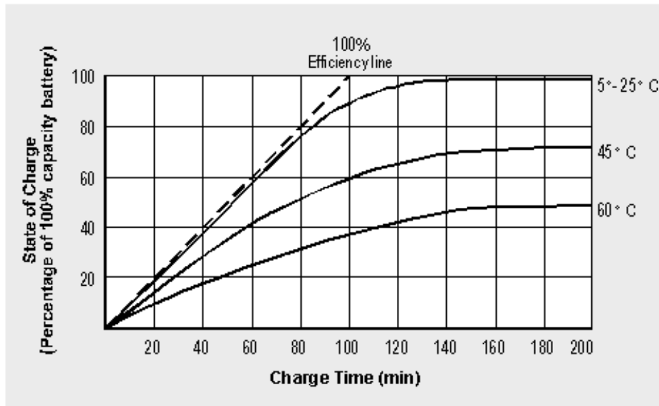
Figure 4-7: Effects of temperature on NiCd charge acceptance. Charge acceptance is much reduced at higher temperatures. NiMH cells follow a similar pattern.
