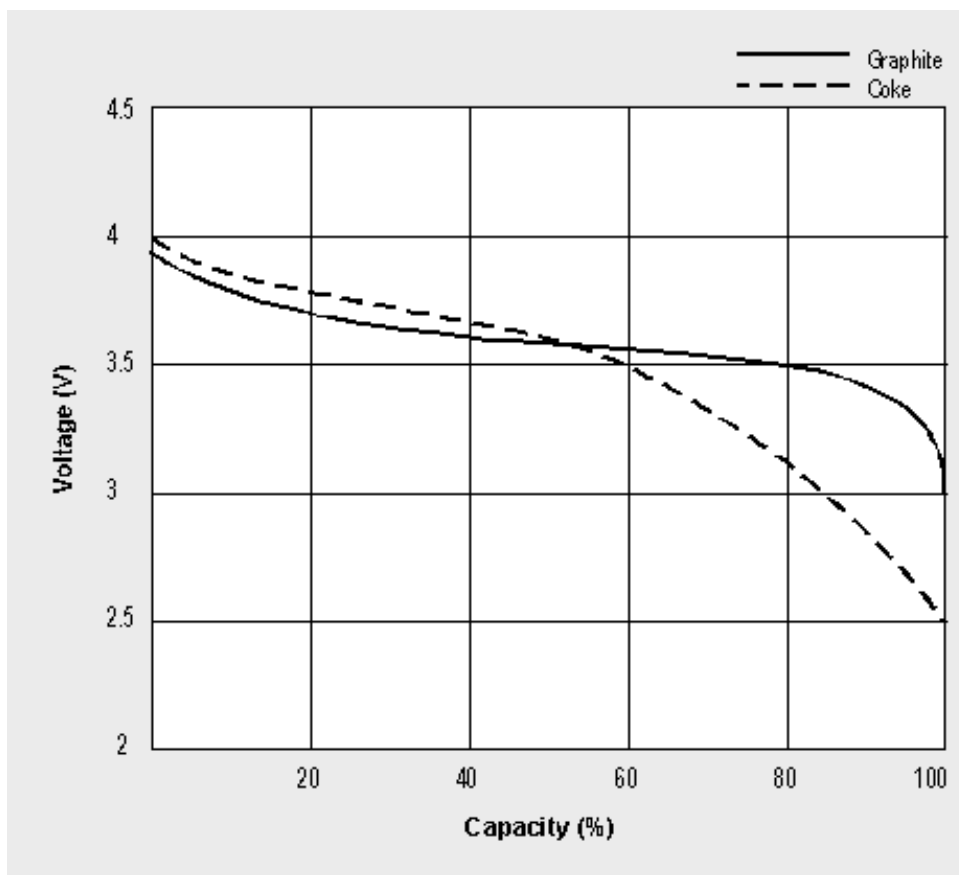
Figure 2-5: Li-ion discharge characteristics.
