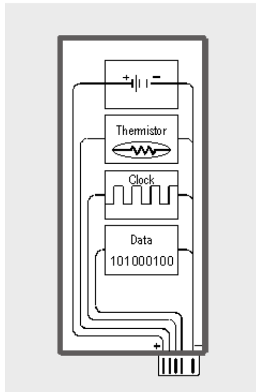
Figure 7-2: Two-wire SMBus system.
