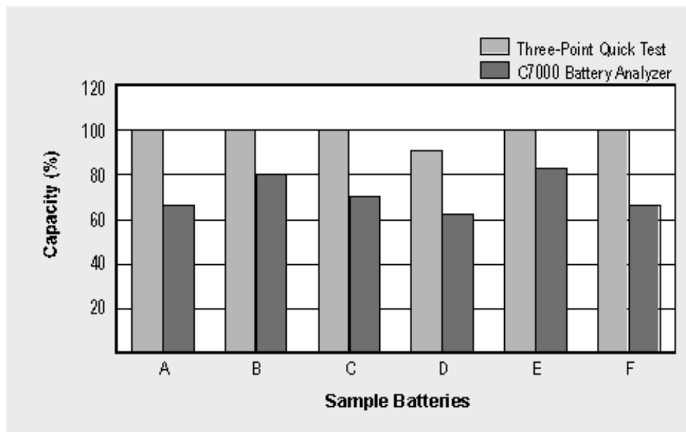
Figure 13-2: Comparison of battery quick test methods.
