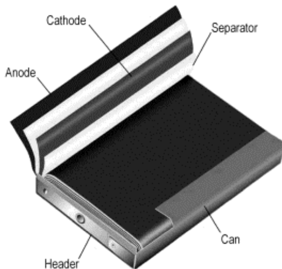
Figure 3-3: Cross-section of a prismatic cell.
