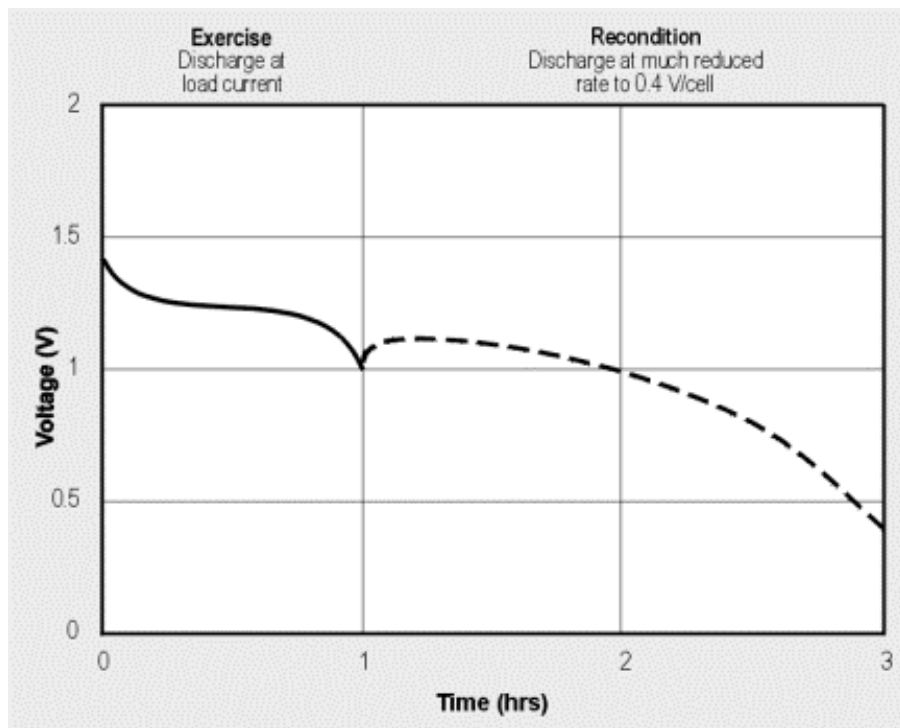
Figure 10-2: Exercising and reconditioning batteries on a Cadex battery analyzer. This illustration shows the battery voltage during a normal discharge to 1V, followed by the secondary discharge (recondition). Recondition consists of a discharge to 1V/cell at a 1C load current, followed by a secondary discharge to 0.4V at a much reduced current. NiCd batteries affected by memory often restore themselves to full service.
