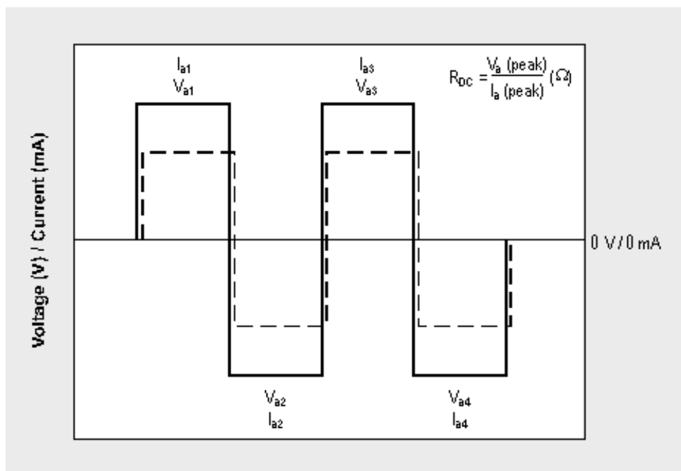
Figure 9-7: Cadex Ohmtest TM .
