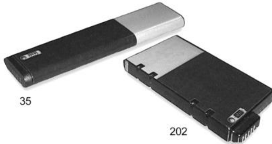
Figure 7-3: 35 and 202 series 'smart' batteries featuring SMBus. Available in NiCd, NiMH and Li-ion chemistries, these batteries are used for mobile computing, biomedical instruments and high-end survey equipment. The same form factor also accommodates NiCd and NiMH chemistries but without SMBus ('dumb').
